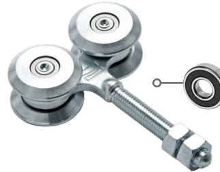
4-WHEEL CARRIER
