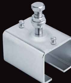
TRACK GUIDE Bolt-on 300-21 Weld-on 300-21-W
