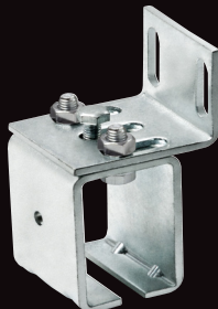
OFFSET GUIDE Bracket & fasteners 300-1BS Track guide 300-2
